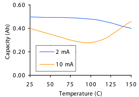
Capacity as a function of current and temperature
