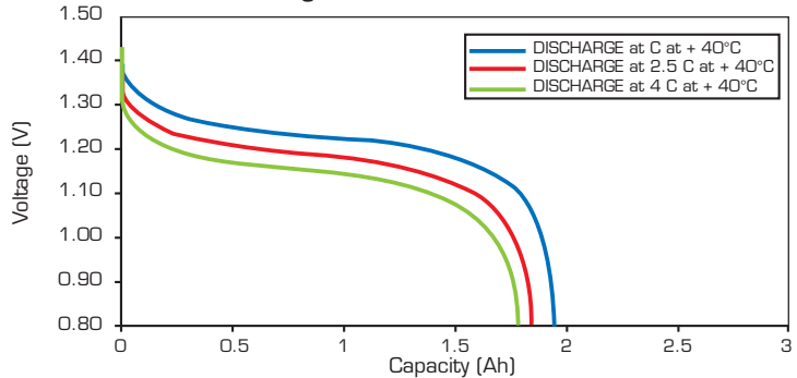
Discharge at + 40°C at different rates
