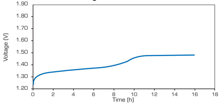
Charge at C/10 at + 40°C
