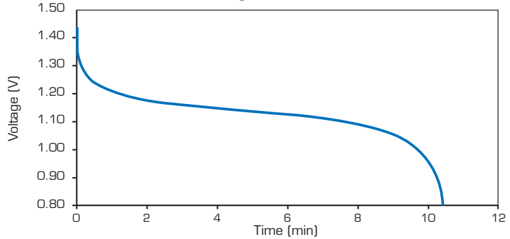
Discharge at 5C at + 40°C
