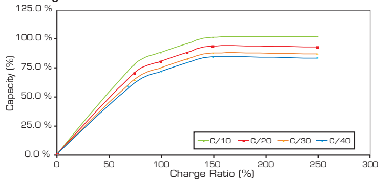
Charge at + 55°C at different rates and different % of charge
