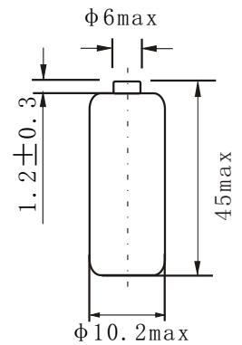
Dimensions in mm S/: STANDARD
